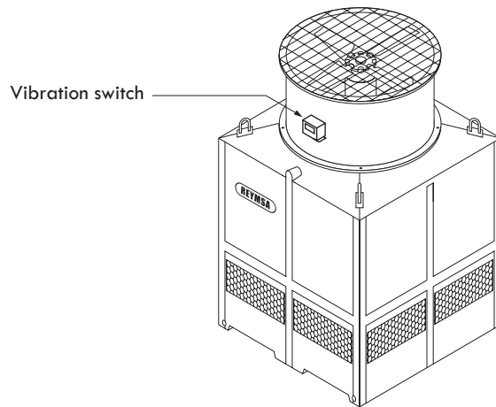
Figure A-48: Vibration Switch recommended location
