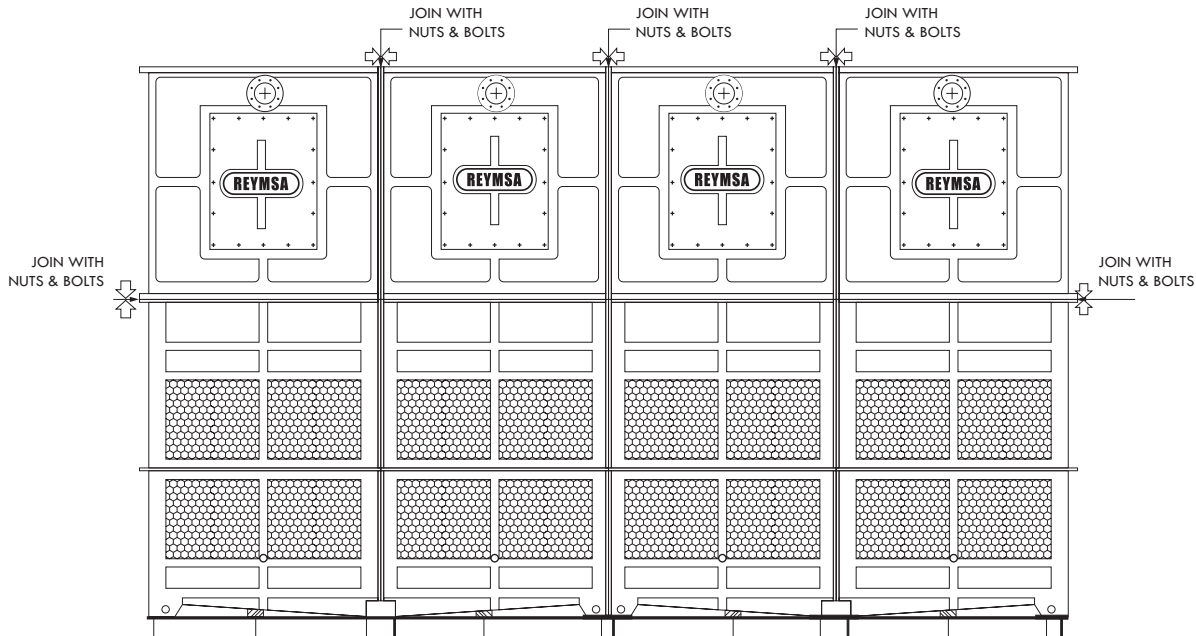
Figure A-29: Tower body section installation
