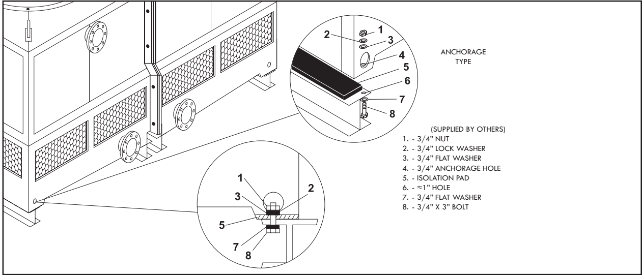
A-18: Installation - Typical anchorage for quadruple fan tower
