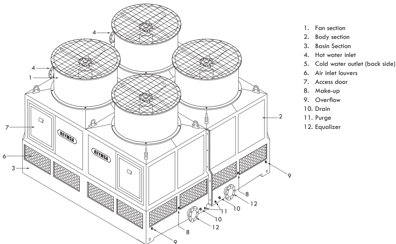
Figure A-62: Quadruple fan cooling tower - Pipe connections
