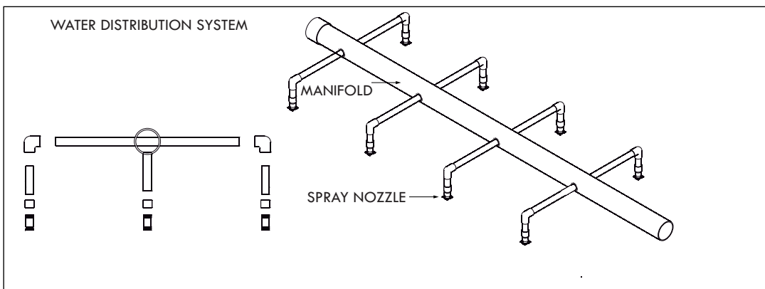
Figura C-1: Water distribution system schematic
