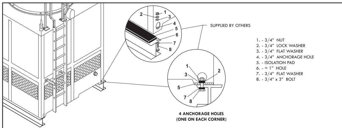
Figure A-6: Installation - Typical anchorage for a single fan tower
