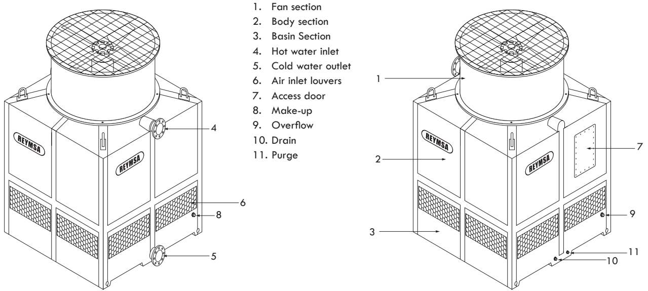
Figure A-60: Single fan cooling tower - Pipe connections
