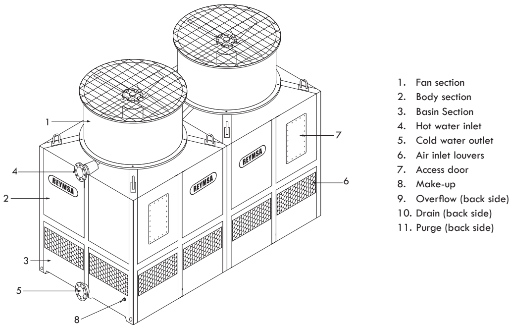
Figure A-61: Double fan cooling tower - Pipe connections
