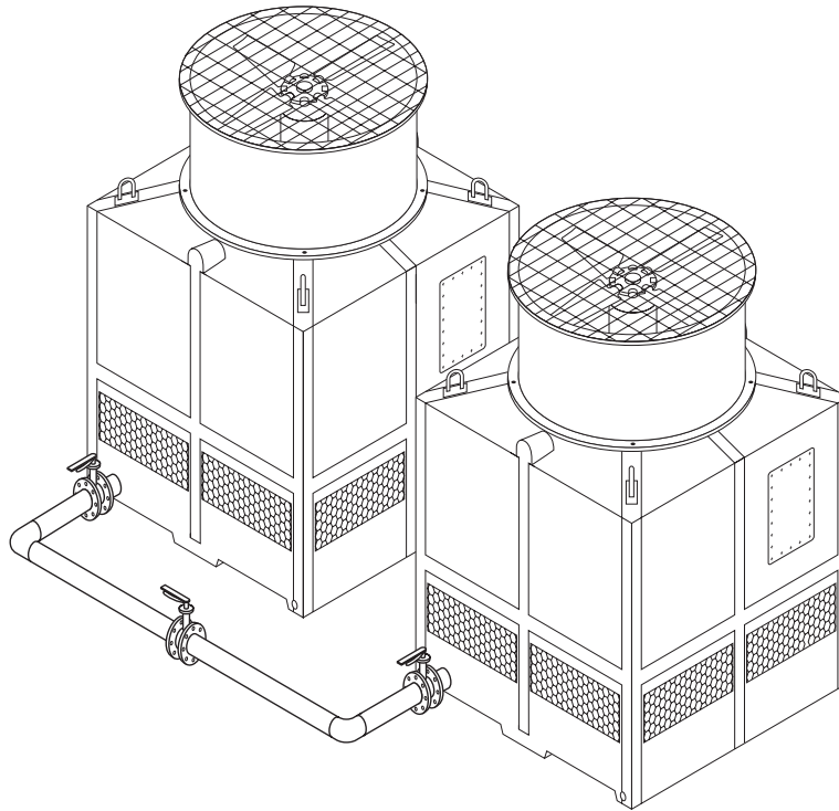
Figure A-63: Example of equalization line
