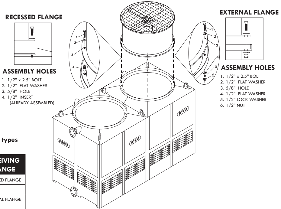
Figure A-13: Fan duct 1 installation - double fan tower
