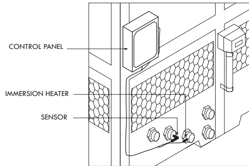
Figure A-53: Basin Heater System
