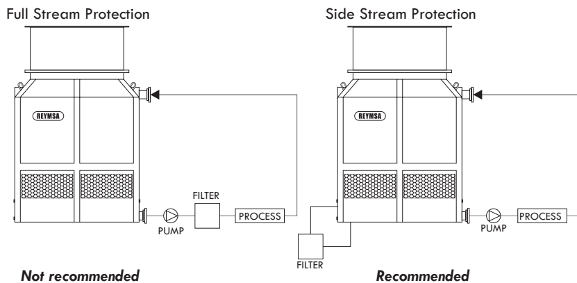
Figure C-2: Filtration system
