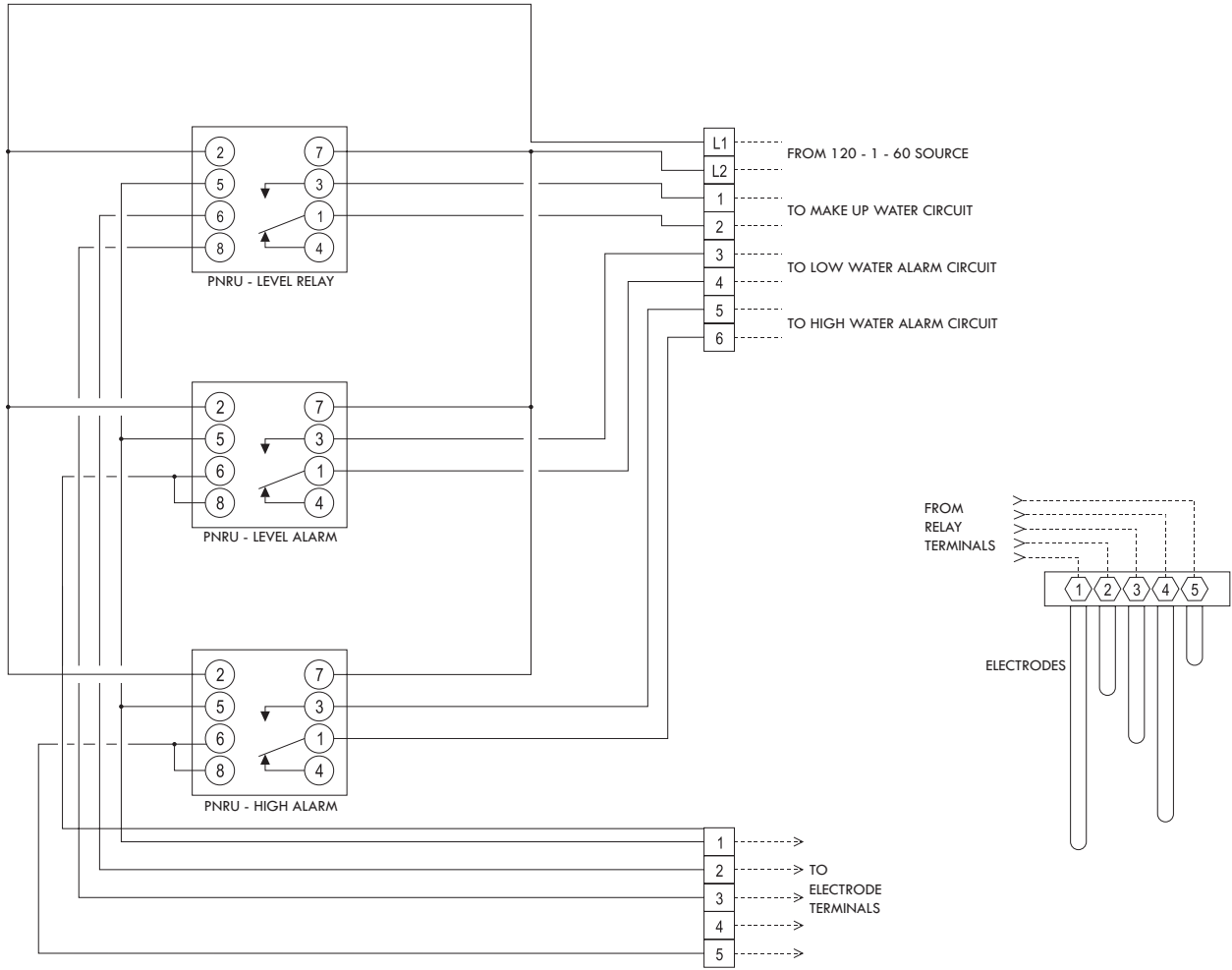
Figure A-58: Water Level and Alarm Controls Diagram
