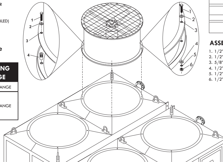
Figure A-20: Fan duct 1 installation for quadruple fan tower
